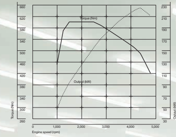
High performance, low emissions – the efficient engine of the BMW xDrive40d.
